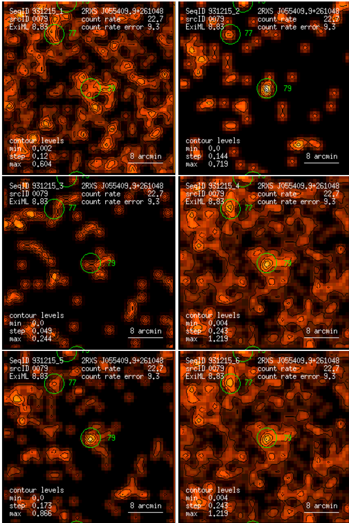
Figure 79: RASS 931215: detection 0079: band rate images, Gaussian filter: (1) PSPC channels 11 – 41, (2) 52 – 90, (3) 91 – 201, (4) 11 – 235, (5) 52 – 201, (6) 11 – 201. Broad band rates in counts/ks. Band rate contour levels in counts/ks/arcmin 2 .
