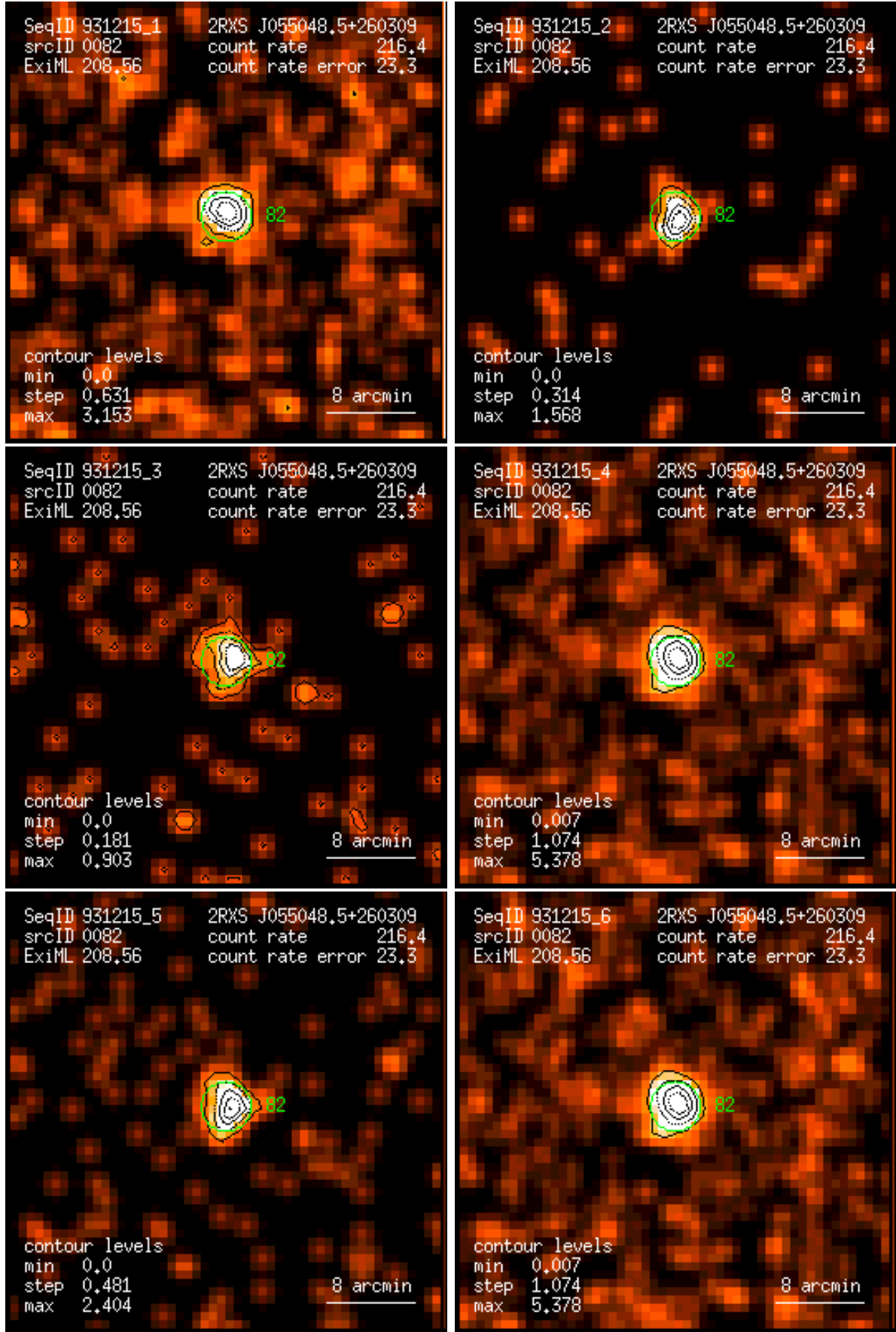
Figure 82: RASS 931215: detection 0082: band rate images, Gaussian filter: (1) PSPC channels 11 – 41, (2) 52 – 90, (3) 91 – 201, (4) 11 – 235, (5) 52 – 201, (6) 11 – 201. Broad band rates in counts/ks. Band rate contour levels in counts/ks/arcmin 2 .
