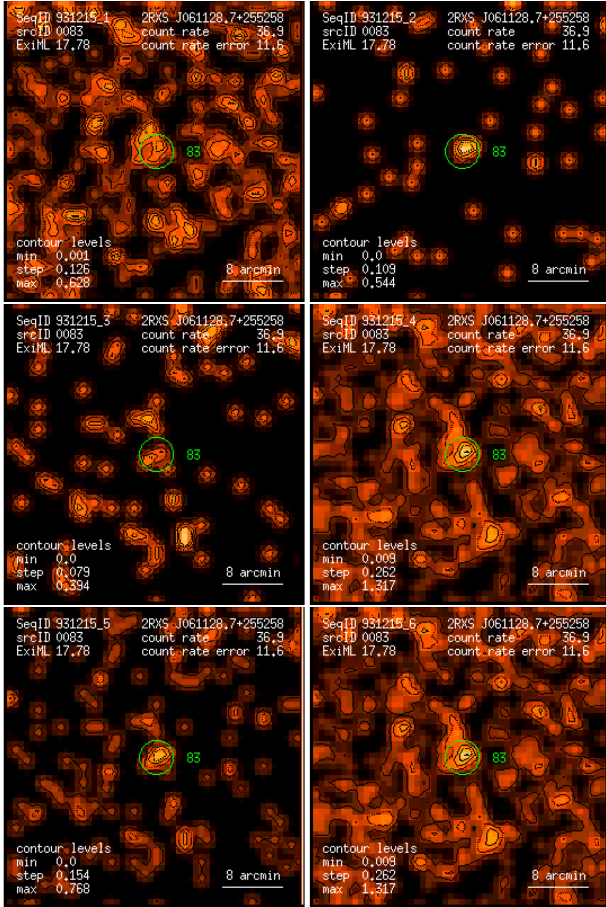
Figure 83: RASS 931215: detection 0083: band rate images, Gaussian filter: (1) PSPC channels 11 – 41, (2) 52 – 90, (3) 91 – 201, (4) 11 – 235, (5) 52 – 201, (6) 11 – 201. Broad band rates in counts/ks. Band rate contour levels in counts/ks/arcmin 2 .
