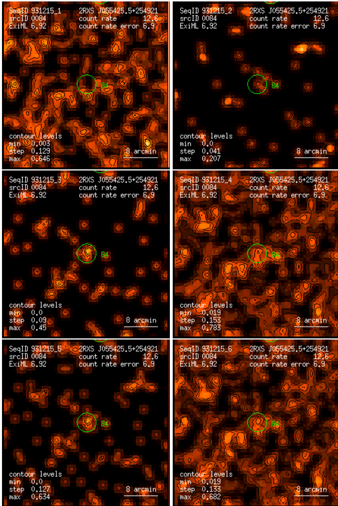
Figure 84: RASS 931215: detection 0084: band rate images, Gaussian filter: (1) PSPC channels 11 – 41, (2) 52 – 90, (3) 91 – 201, (4) 11 – 235, (5) 52 – 201, (6) 11 – 201. Broad band rates in counts/ks. Band rate contour levels in counts/ks/arcmin 2 .
