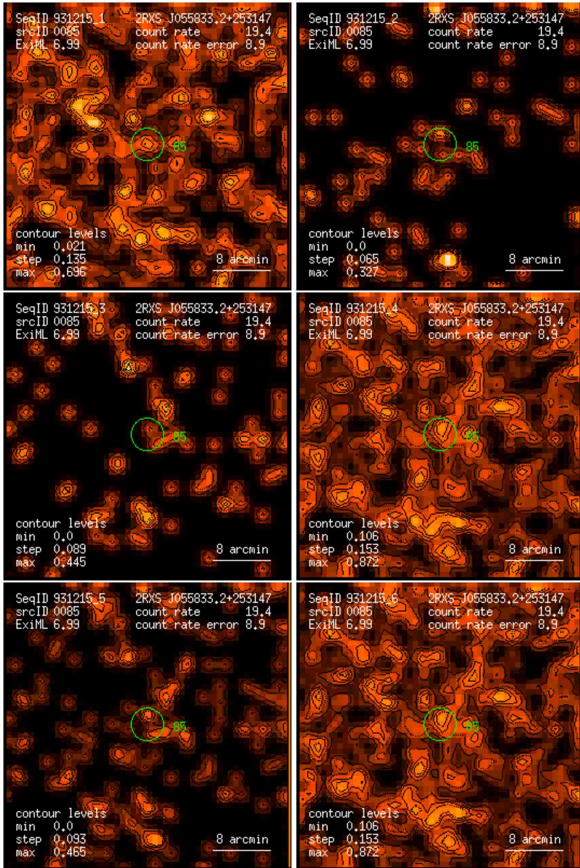
Figure 85: RASS 931215: detection 0085: band rate images, Gaussian filter: (1) PSPC channels 11 – 41, (2) 52 – 90, (3) 91 – 201, (4) 11 – 235, (5) 52 – 201, (6) 11 – 201. Broad band rates in counts/ks. Band rate contour levels in counts/ks/arcmin 2 .
