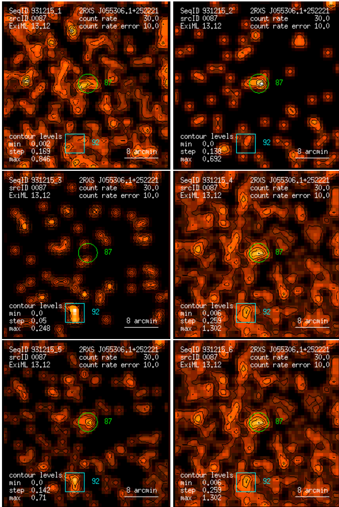
Figure 87: RASS 931215: detection 0087: band rate images, Gaussian filter: (1) PSPC channels 11 – 41, (2) 52 – 90, (3) 91 – 201, (4) 11 – 235, (5) 52 – 201, (6) 11 – 201. Broad band rates in counts/ks. Band rate contour levels in counts/ks/arcmin 2 .
