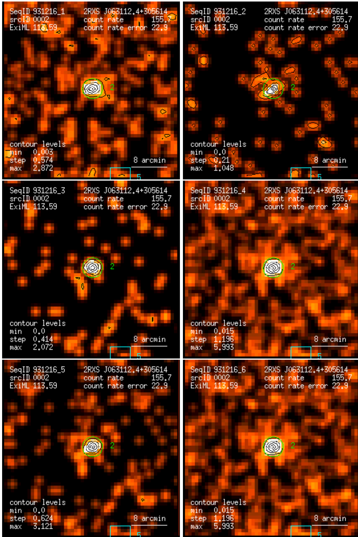
Figure 2: RASS 931216: detection 0002: band rate images, Gaussian filter: (1) PSPC channels 11 – 41, (2) 52 – 90, (3) 91 – 201, (4) 11 – 235, (5) 52 – 201, (6) 11 – 201. Broad band rates in counts/ks. Band rate contour levels in counts/ks/arcmin 2 .
