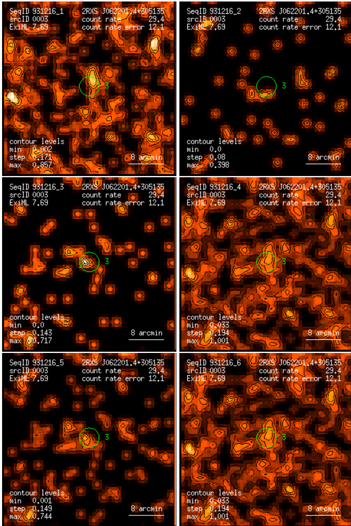
Figure 3: RASS 931216: detection 0003: band rate images, Gaussian filter: (1) PSPC channels 11 – 41, (2) 52 – 90, (3) 91 – 201, (4) 11 – 235, (5) 52 – 201, (6) 11 – 201. Broad band rates in counts/ks. Band rate contour levels in counts/ks/arcmin 2 .
