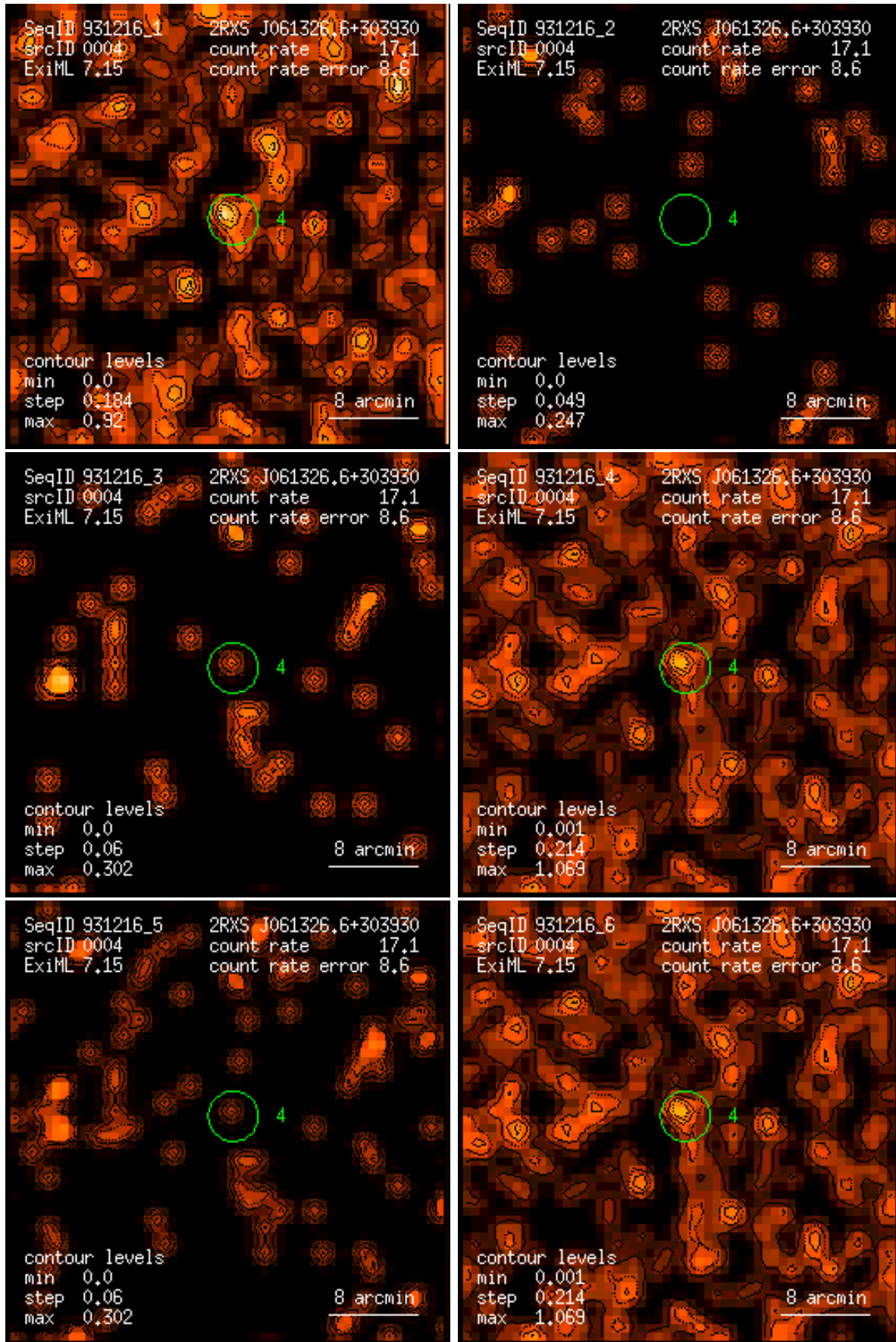
Figure 4: RASS 931216: detection 0004: band rate images, Gaussian filter: (1) PSPC channels 11 – 41, (2) 52 – 90, (3) 91 – 201, (4) 11 – 235, (5) 52 – 201, (6) 11 – 201. Broad band rates in counts/ks. Band rate contour levels in counts/ks/arcmin 2 .
