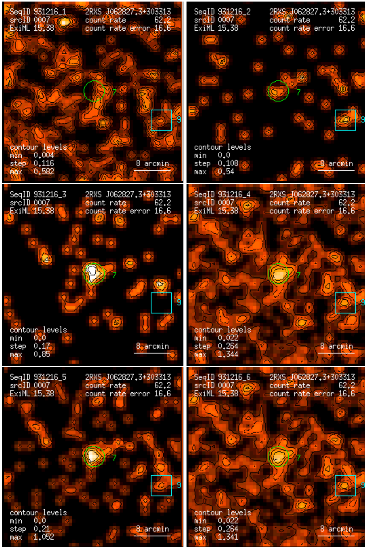
Figure 7: RASS 931216: detection 0007: band rate images, Gaussian filter: (1) PSPC channels 11 – 41, (2) 52 – 90, (3) 91 – 201, (4) 11 – 235, (5) 52 – 201, (6) 11 – 201. Broad band rates in counts/ks. Band rate contour levels in counts/ks/arcmin 2 .
