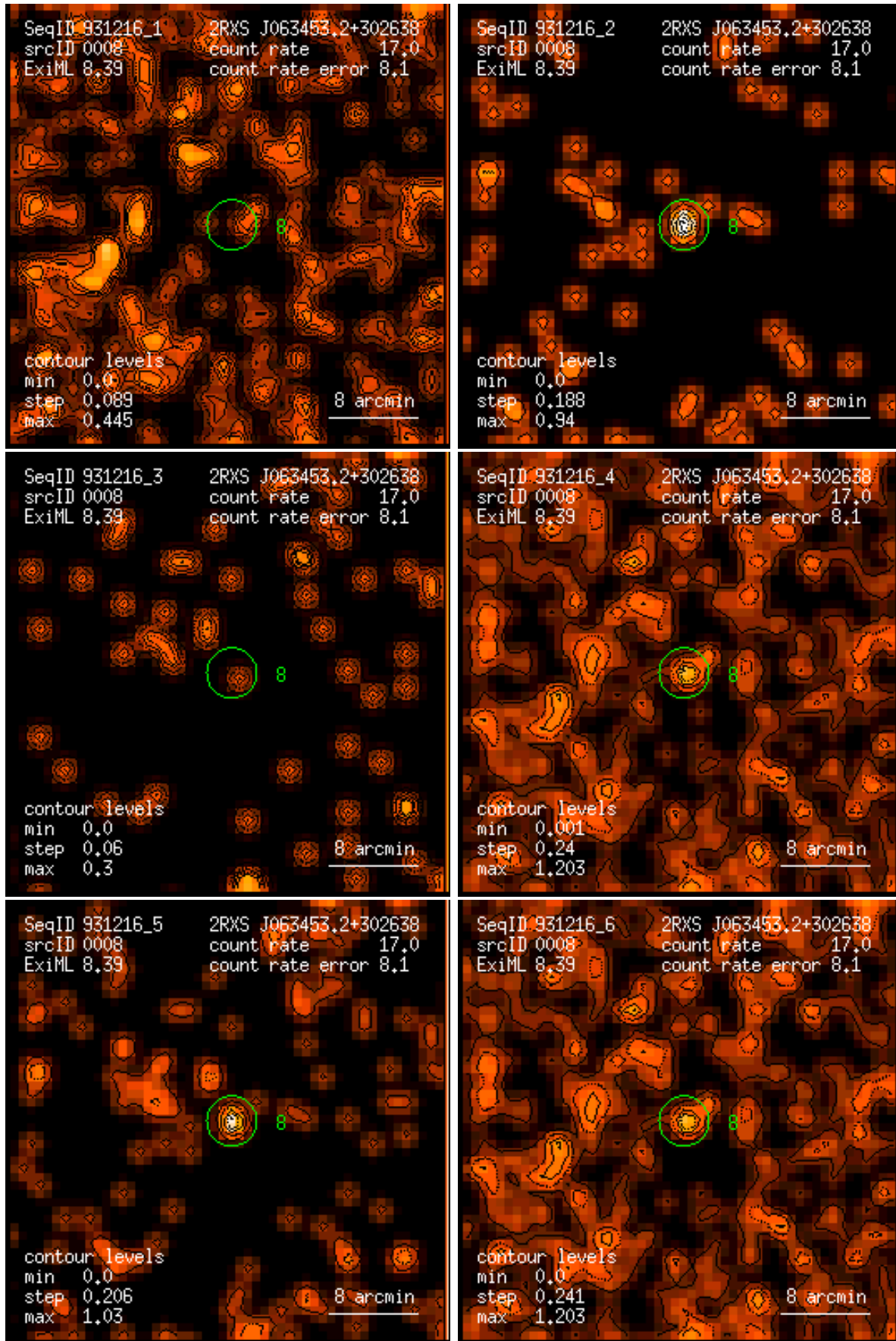
Figure 8: RASS 931216: detection 0008: band rate images, Gaussian filter: (1) PSPC channels 11 – 41, (2) 52 – 90, (3) 91 – 201, (4) 11 – 235, (5) 52 – 201, (6) 11 – 201. Broad band rates in counts/ks. Band rate contour levels in counts/ks/arcmin 2 .
