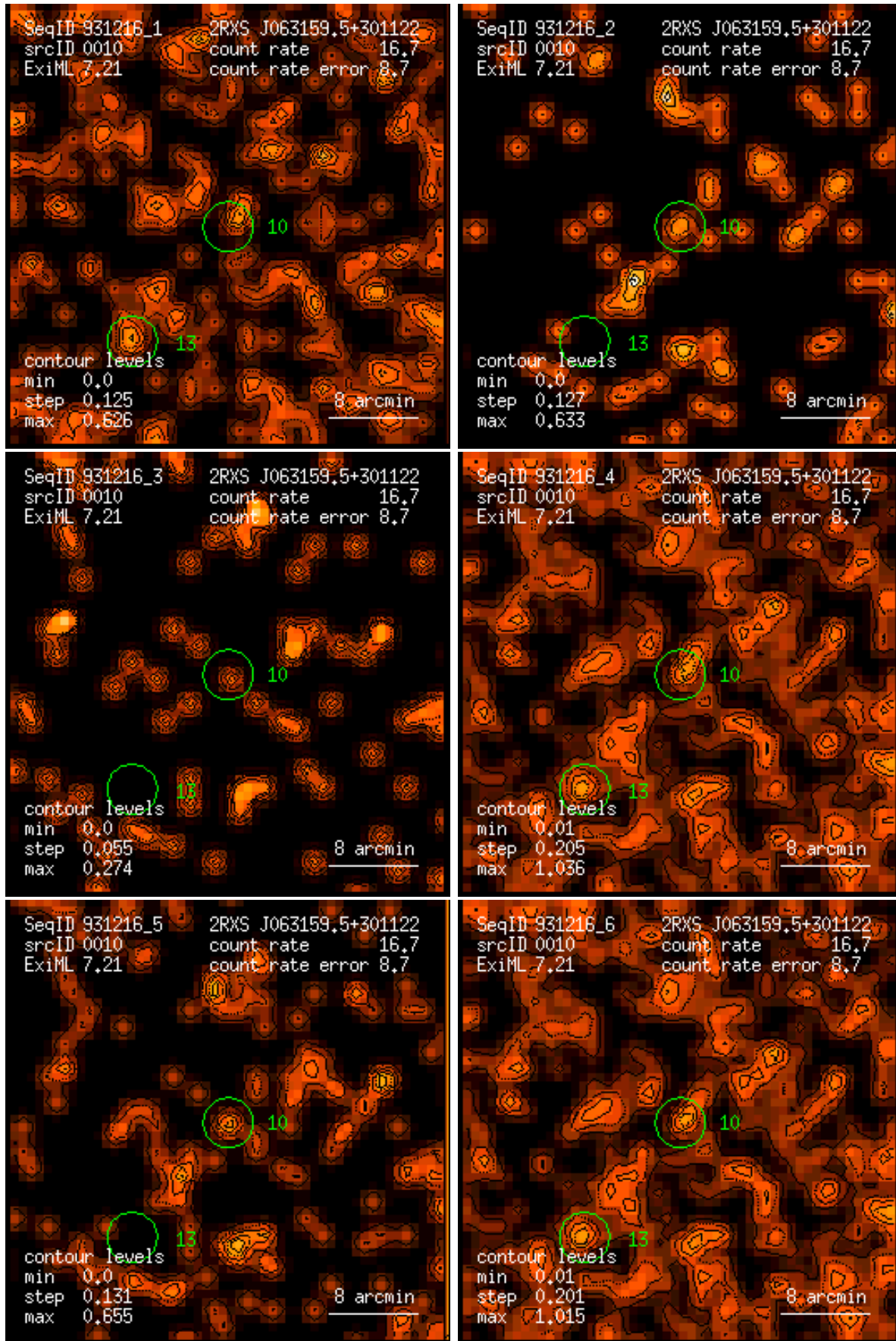
Figure 10: RASS 931216: detection 0010: band rate images, Gaussian filter: (1) PSPC channels 11 – 41, (2) 52 – 90, (3) 91 – 201, (4) 11 – 235, (5) 52 – 201, (6) 11 – 201. Broad band rates in counts/ks. Band rate contour levels in counts/ks/arcmin 2 .
