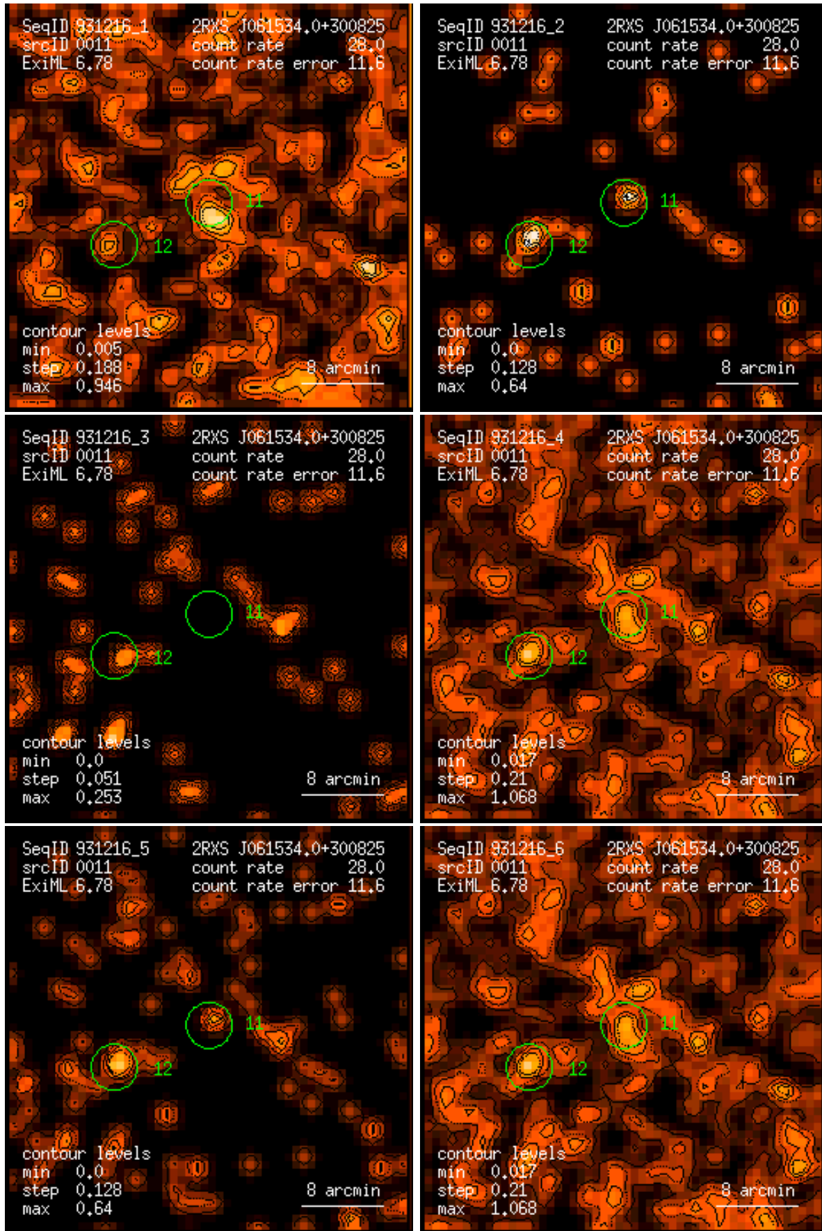
Figure 11: RASS 931216: detection 0011: band rate images, Gaussian filter: (1) PSPC channels 11 – 41, (2) 52 – 90, (3) 91 – 201, (4) 11 – 235, (5) 52 – 201, (6) 11 – 201. Broad band rates in counts/ks. Band rate contour levels in counts/ks/arcmin 2 .
