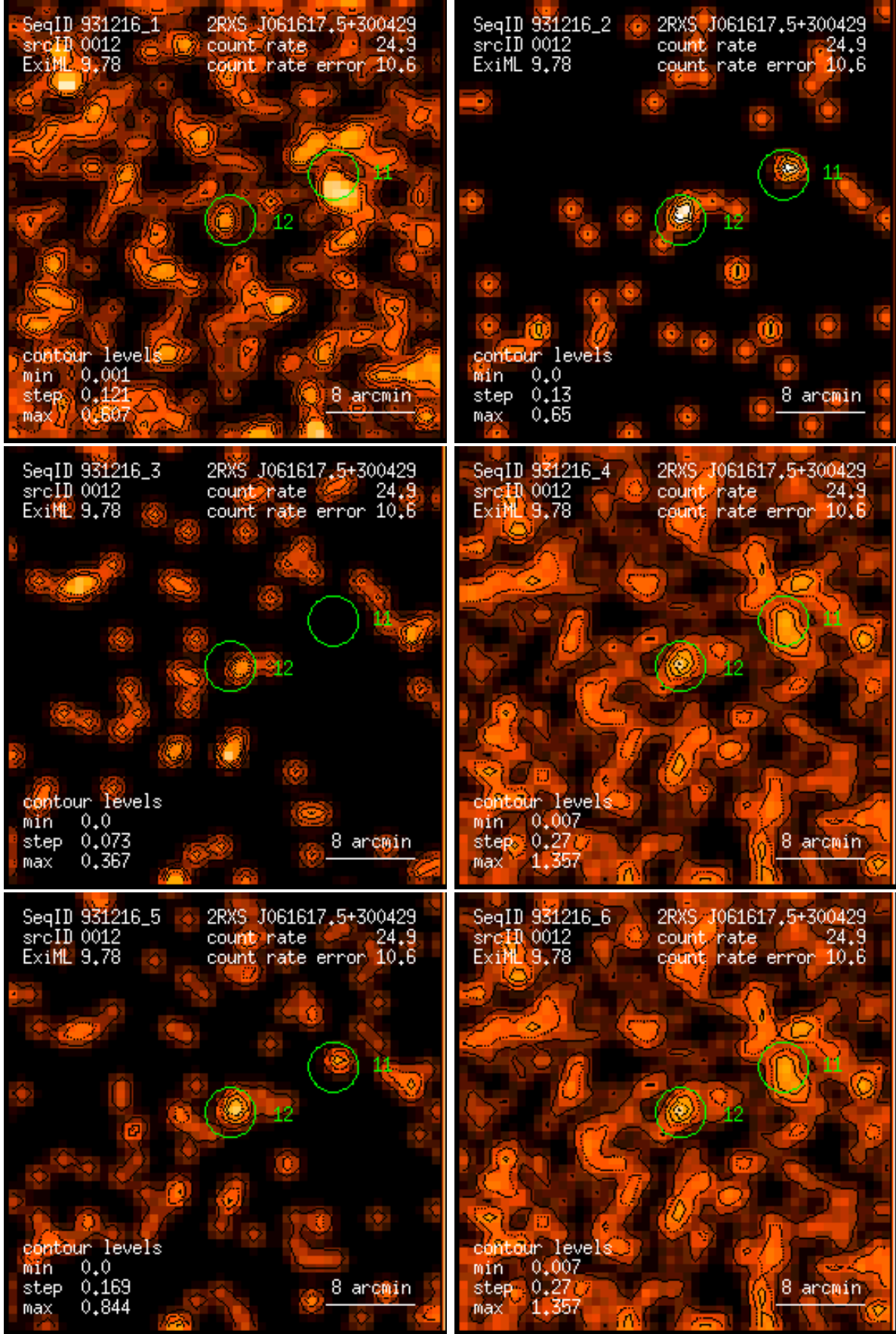
Figure 12: RASS 931216: detection 0012: band rate images, Gaussian filter: (1) PSPC channels 11 – 41, (2) 52 – 90, (3) 91 – 201, (4) 11 – 235, (5) 52 – 201, (6) 11 – 201. Broad band rates in counts/ks. Band rate contour levels in counts/ks/arcmin 2 .
