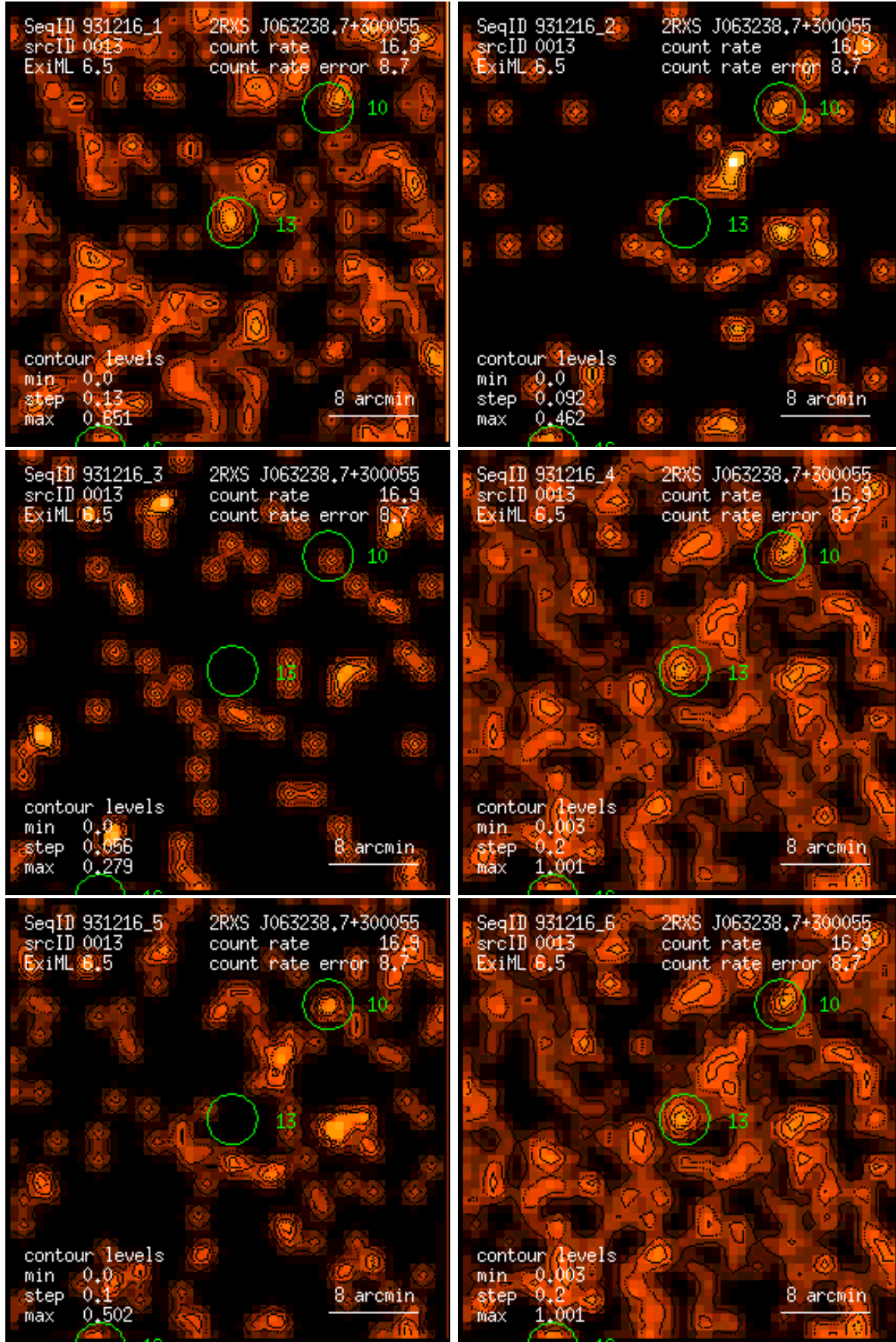
Figure 13: RASS 931216: detection 0013: band rate images, Gaussian filter: (1) PSPC channels 11 – 41, (2) 52 – 90, (3) 91 – 201, (4) 11 – 235, (5) 52 – 201, (6) 11 – 201. Broad band rates in counts/ks. Band rate contour levels in counts/ks/arcmin 2 .
