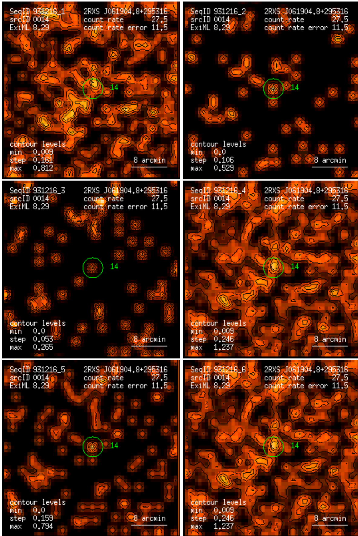
Figure 14: RASS 931216: detection 0014: band rate images, Gaussian filter: (1) PSPC channels 11 – 41, (2) 52 – 90, (3) 91 – 201, (4) 11 – 235, (5) 52 – 201, (6) 11 – 201. Broad band rates in counts/ks. Band rate contour levels in counts/ks/arcmin 2 .
