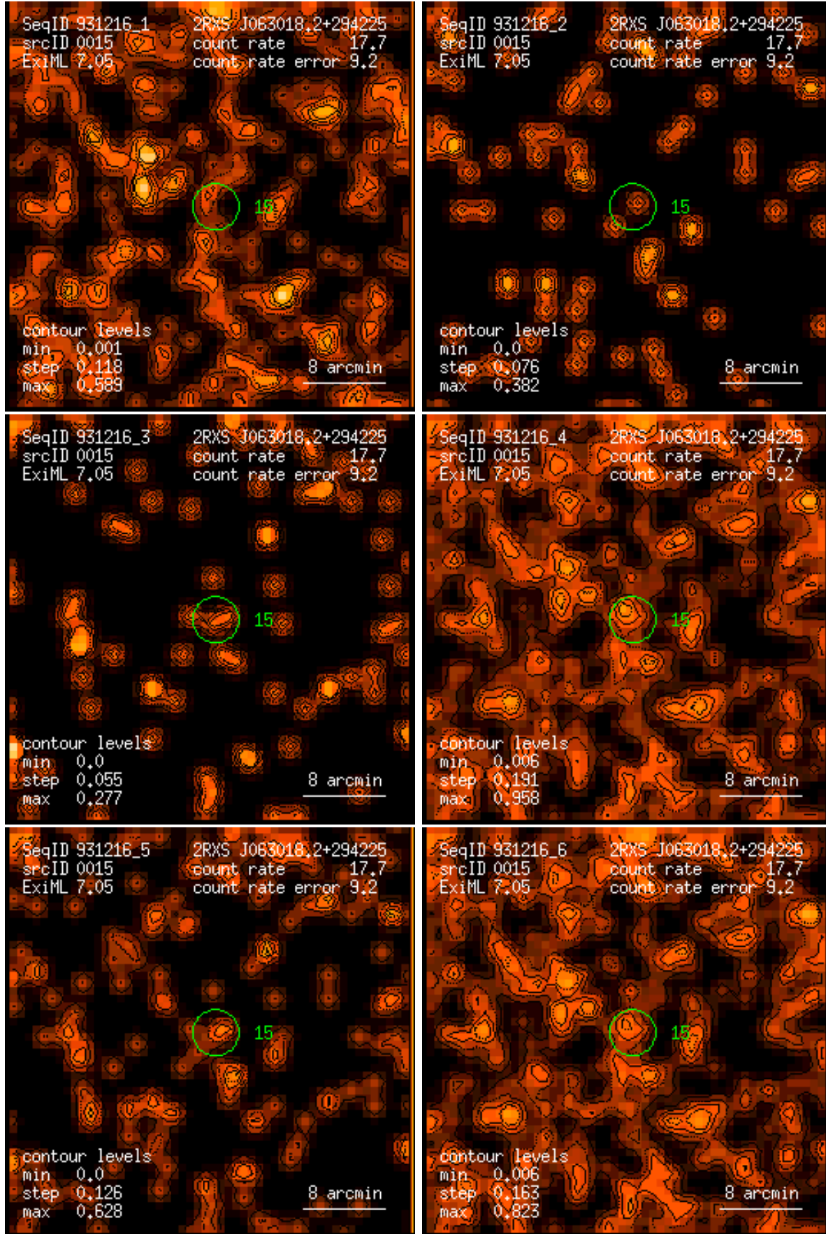
Figure 15: RASS 931216: detection 0015: band rate images, Gaussian filter: (1) PSPC channels 11 – 41, (2) 52 – 90, (3) 91 – 201, (4) 11 – 235, (5) 52 – 201, (6) 11 – 201. Broad band rates in counts/ks. Band rate contour levels in counts/ks/arcmin 2 .
