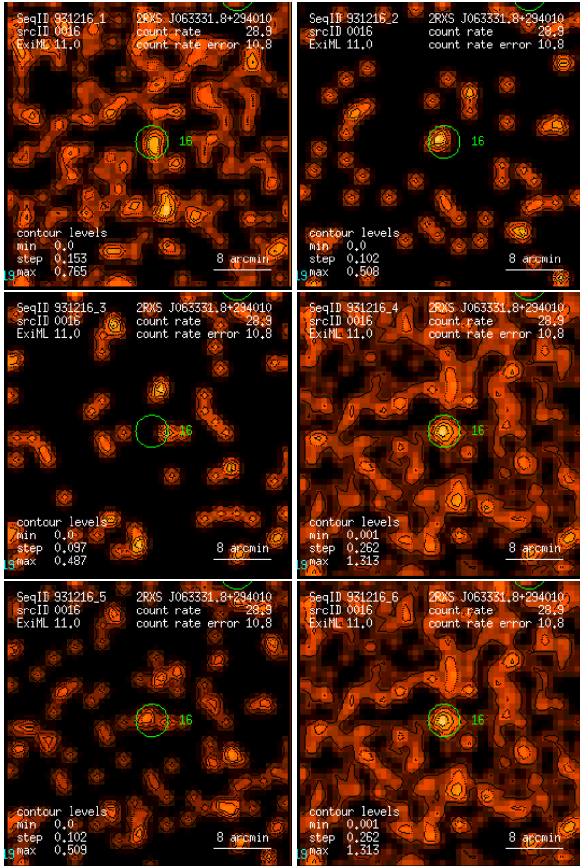
Figure 16: RASS 931216: detection 0016: band rate images, Gaussian filter: (1) PSPC channels 11 – 41, (2) 52 – 90, (3) 91 – 201, (4) 11 – 235, (5) 52 – 201, (6) 11 – 201. Broad band rates in counts/ks. Band rate contour levels in counts/ks/arcmin 2 .
