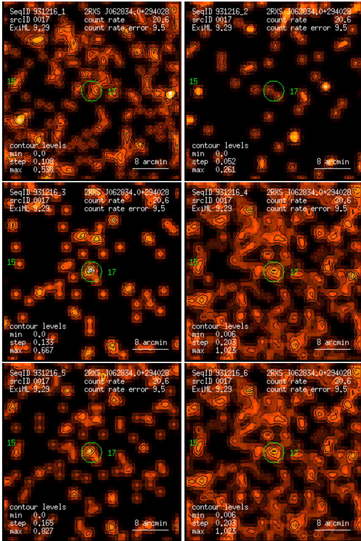
Figure 17: RASS 931216: detection 0017: band rate images, Gaussian filter: (1) PSPC channels 11 – 41, (2) 52 – 90, (3) 91 – 201, (4) 11 – 235, (5) 52 – 201, (6) 11 – 201. Broad band rates in counts/ks. Band rate contour levels in counts/ks/arcmin 2 .
