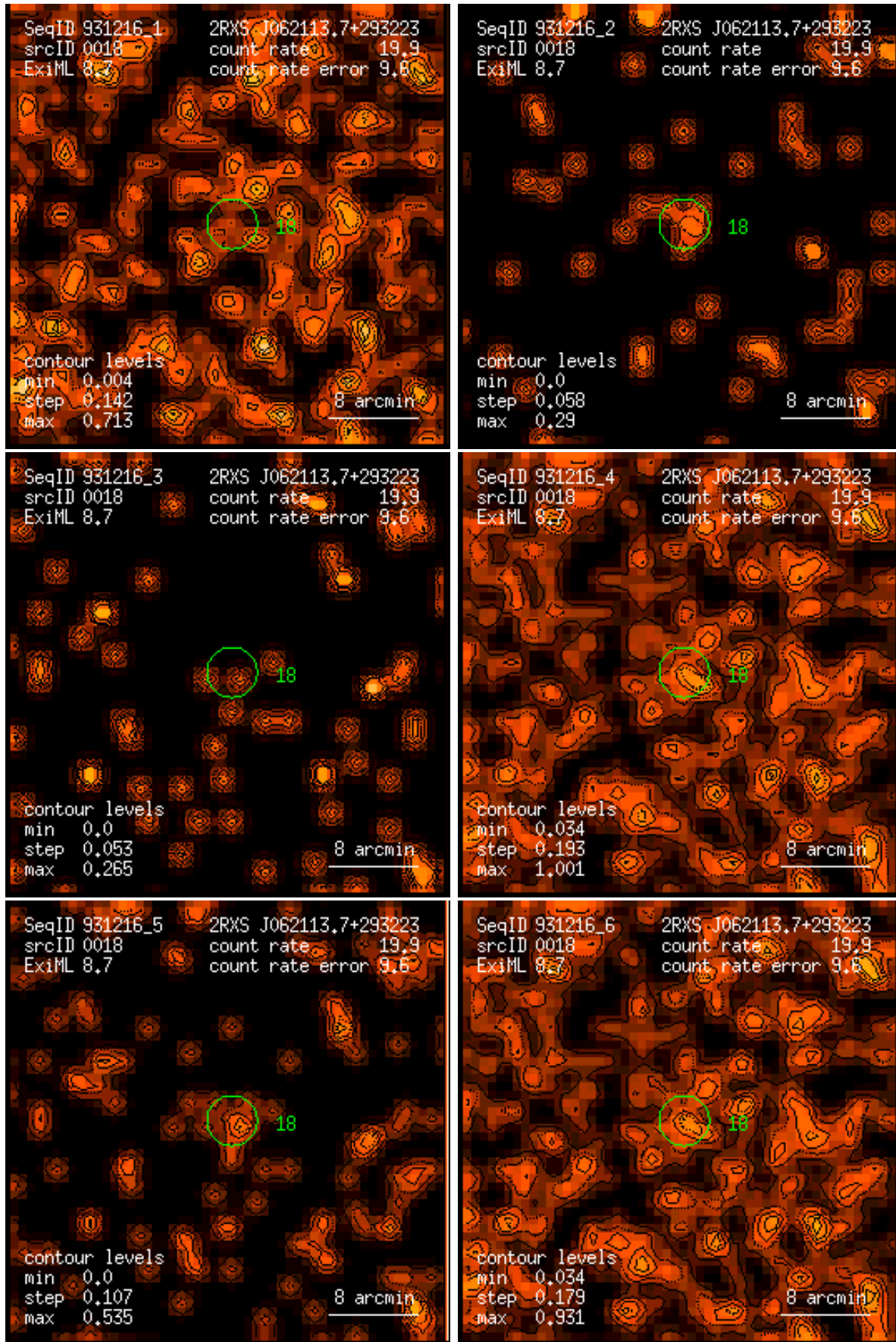
Figure 18: RASS 931216: detection 0018: band rate images, Gaussian filter: (1) PSPC channels 11 – 41, (2) 52 – 90, (3) 91 – 201, (4) 11 – 235, (5) 52 – 201, (6) 11 – 201. Broad band rates in counts/ks. Band rate contour levels in counts/ks/arcmin 2 .
