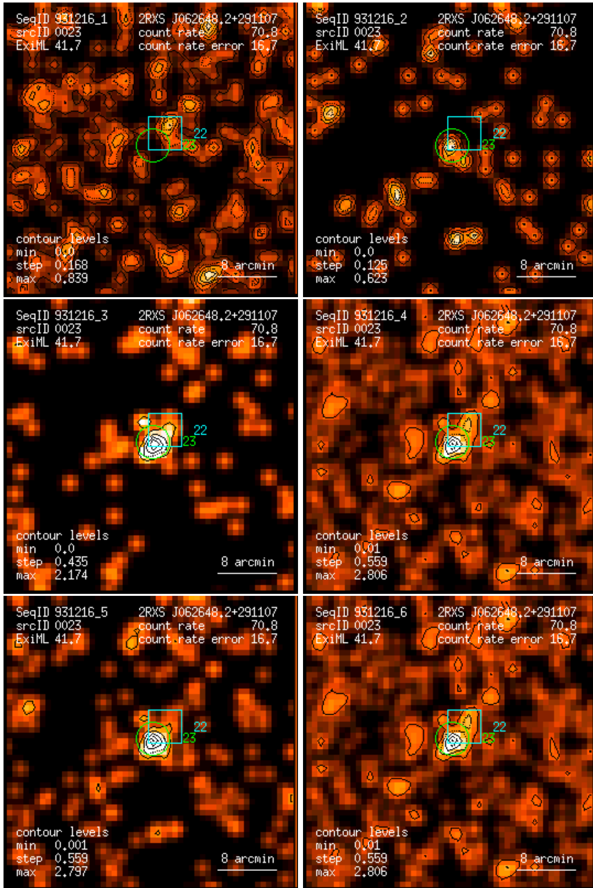
Figure 23: RASS 931216: detection 0023: band rate images, Gaussian filter: (1) PSPC channels 11 – 41, (2) 52 – 90, (3) 91 – 201, (4) 11 – 235, (5) 52 – 201, (6) 11 – 201. Broad band rates in counts/ks. Band rate contour levels in counts/ks/arcmin 2 .
