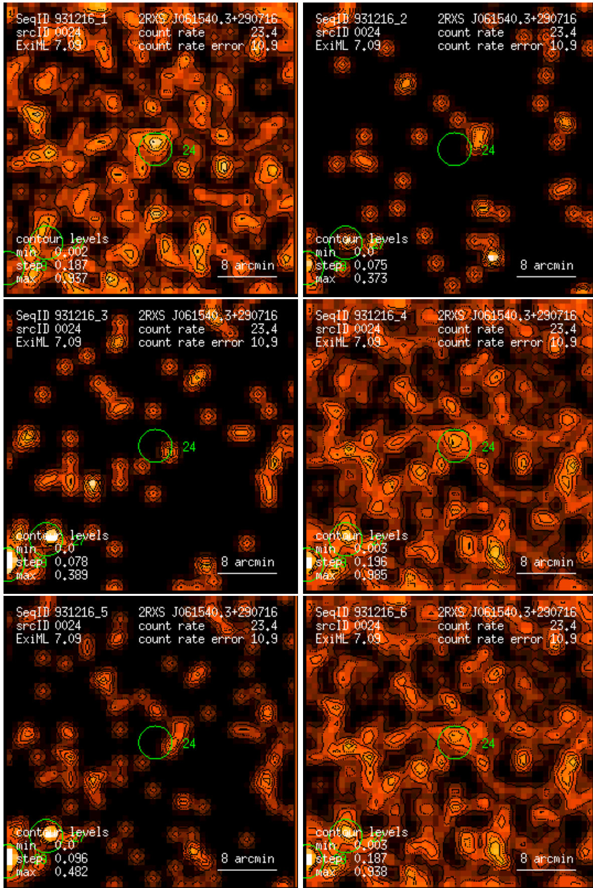
Figure 24: RASS 931216: detection 0024: band rate images, Gaussian filter: (1) PSPC channels 11 – 41, (2) 52 – 90, (3) 91 – 201, (4) 11 – 235, (5) 52 – 201, (6) 11 – 201. Broad band rates in counts/ks. Band rate contour levels in counts/ks/arcmin 2 .
