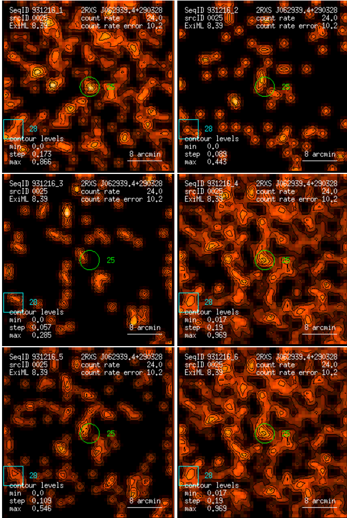
Figure 25: RASS 931216: detection 0025: band rate images, Gaussian filter: (1) PSPC channels 11 – 41, (2) 52 – 90, (3) 91 – 201, (4) 11 – 235, (5) 52 – 201, (6) 11 – 201. Broad band rates in counts/ks. Band rate contour levels in counts/ks/arcmin 2 .
