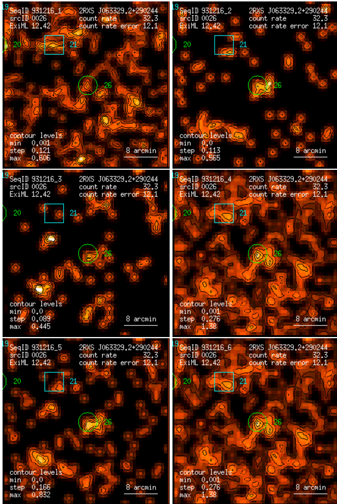
Figure 26: RASS 931216: detection 0026: band rate images, Gaussian filter: (1) PSPC channels 11 – 41, (2) 52 – 90, (3) 91 – 201, (4) 11 – 235, (5) 52 – 201, (6) 11 – 201. Broad band rates in counts/ks. Band rate contour levels in counts/ks/arcmin 2 .
