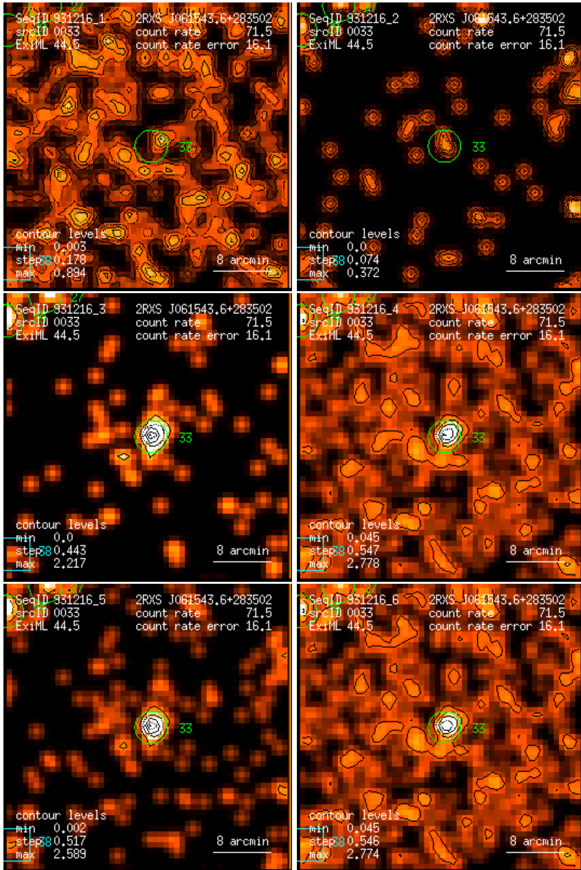
Figure 33: RASS 931216: detection 0033: band rate images, Gaussian filter: (1) PSPC channels 11 – 41, (2) 52 – 90, (3) 91 – 201, (4) 11 – 235, (5) 52 – 201, (6) 11 – 201. Broad band rates in counts/ks. Band rate contour levels in counts/ks/arcmin 2 .
