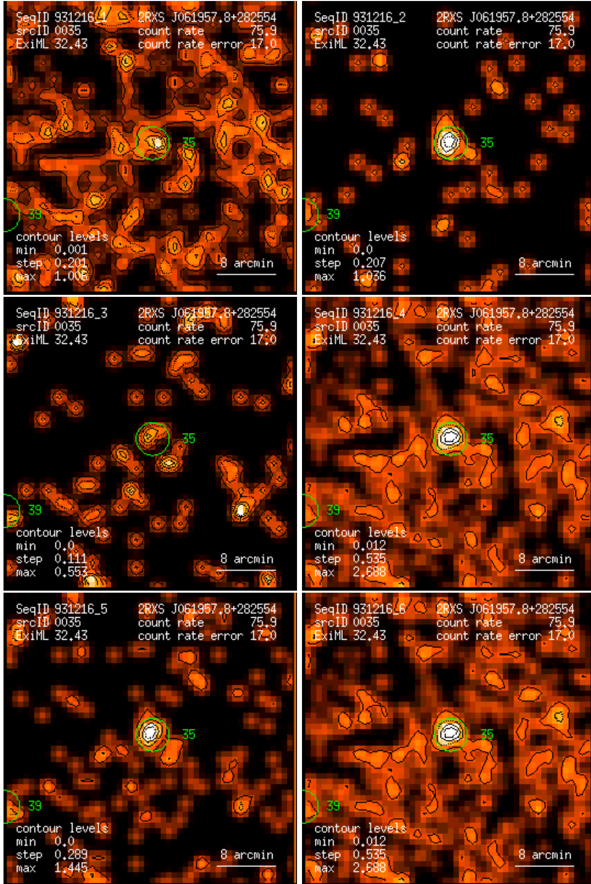
Figure 35: RASS 931216: detection 0035: band rate images, Gaussian filter: (1) PSPC channels 11 – 41, (2) 52 – 90, (3) 91 – 201, (4) 11 – 235, (5) 52 – 201, (6) 11 – 201. Broad band rates in counts/ks. Band rate contour levels in counts/ks/arcmin 2 .
