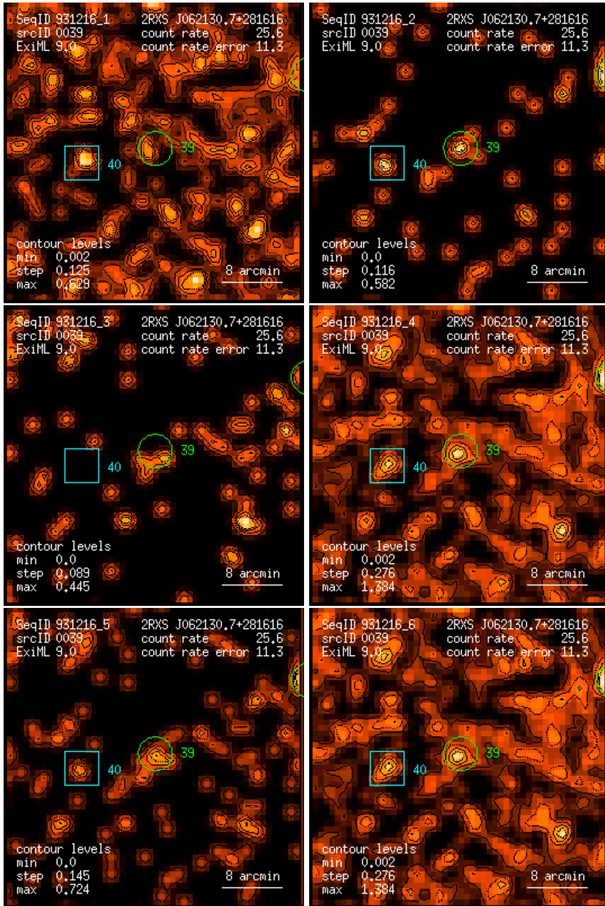
Figure 39: RASS 931216: detection 0039: band rate images, Gaussian filter: (1) PSPC channels 11 – 41, (2) 52 – 90, (3) 91 – 201, (4) 11 – 235, (5) 52 – 201, (6) 11 – 201. Broad band rates in counts/ks. Band rate contour levels in counts/ks/arcmin 2 .
