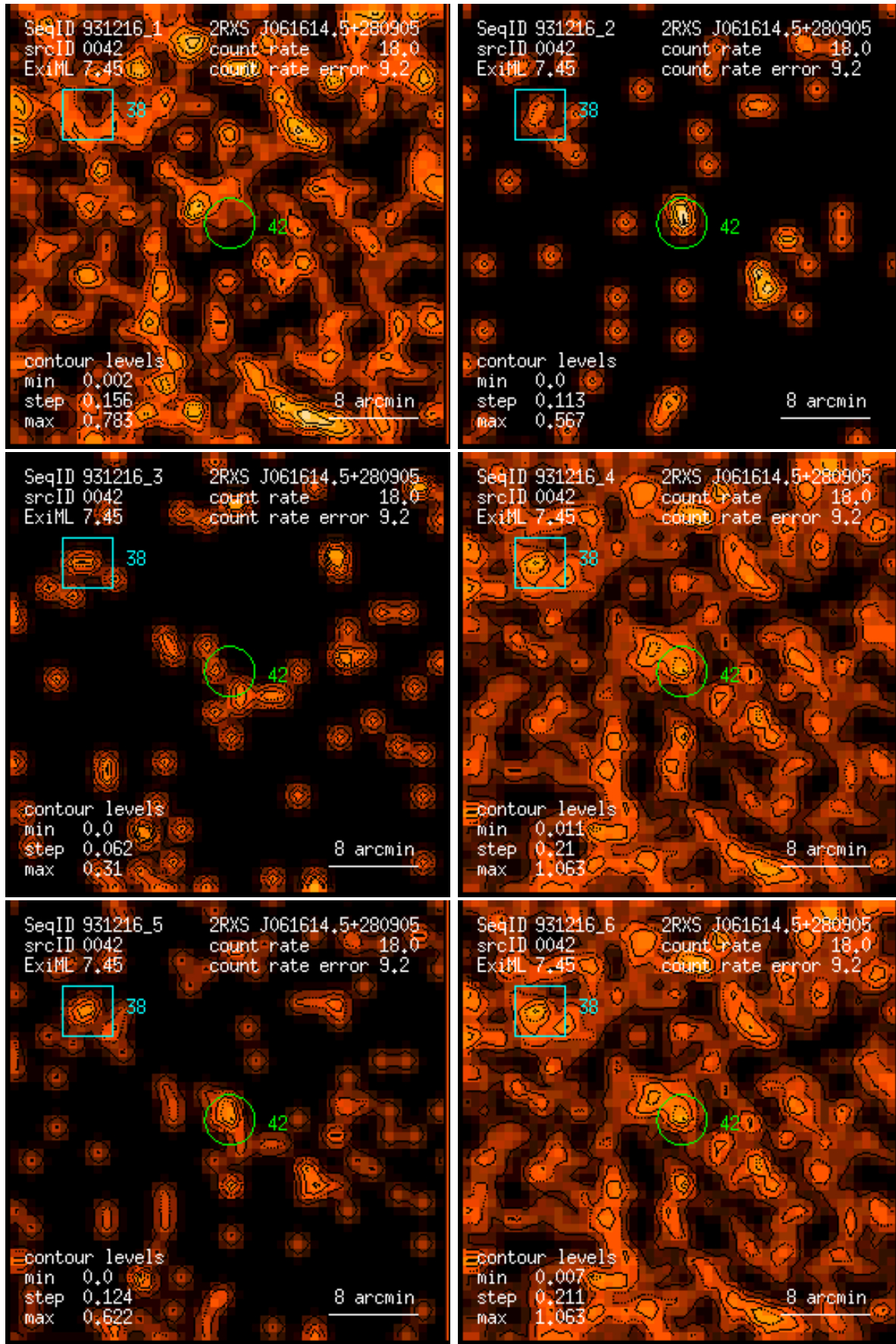
Figure 42: RASS 931216: detection 0042: band rate images, Gaussian filter: (1) PSPC channels 11 – 41, (2) 52 – 90, (3) 91 – 201, (4) 11 – 235, (5) 52 – 201, (6) 11 – 201. Broad band rates in counts/ks. Band rate contour levels in counts/ks/arcmin 2 .
