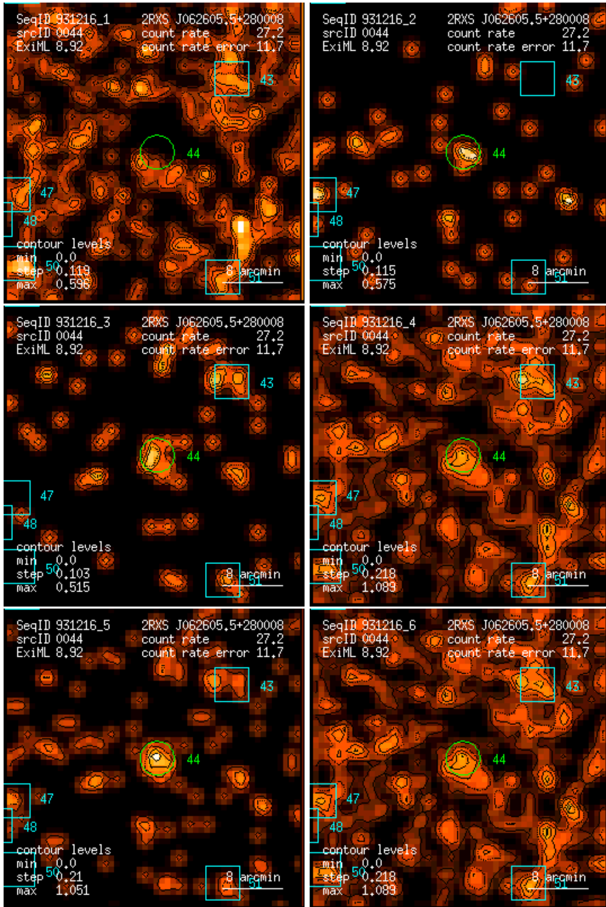
Figure 44: RASS 931216: detection 0044: band rate images, Gaussian filter: (1) PSPC channels 11 – 41, (2) 52 – 90, (3) 91 – 201, (4) 11 – 235, (5) 52 – 201, (6) 11 – 201. Broad band rates in counts/ks. Band rate contour levels in counts/ks/arcmin 2 .
