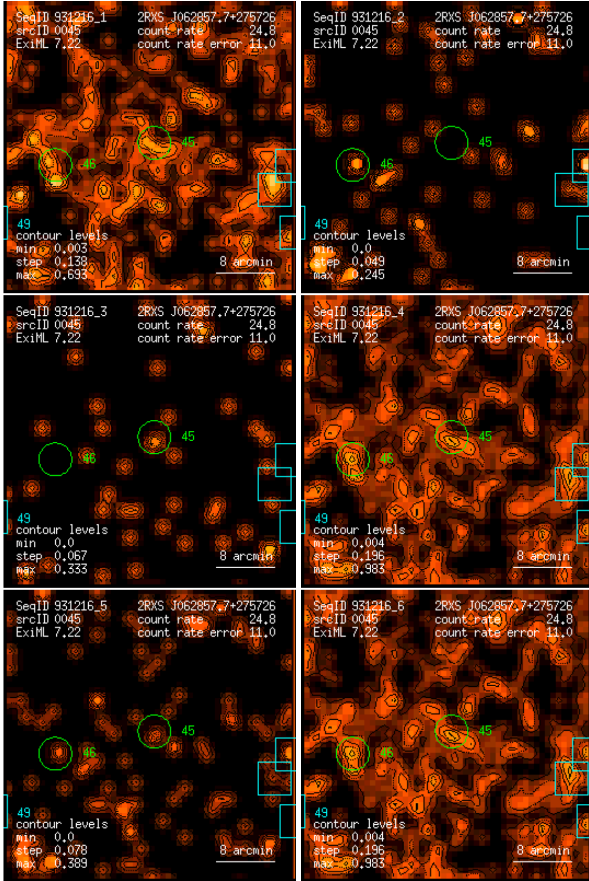
Figure 45: RASS 931216: detection 0045: band rate images, Gaussian filter: (1) PSPC channels 11 – 41, (2) 52 – 90, (3) 91 – 201, (4) 11 – 235, (5) 52 – 201, (6) 11 – 201. Broad band rates in counts/ks. Band rate contour levels in counts/ks/arcmin 2 .
