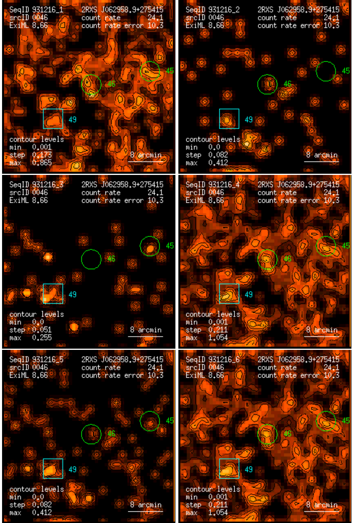
Figure 46: RASS 931216: detection 0046: band rate images, Gaussian filter: (1) PSPC channels 11 – 41, (2) 52 – 90, (3) 91 – 201, (4) 11 – 235, (5) 52 – 201, (6) 11 – 201. Broad band rates in counts/ks. Band rate contour levels in counts/ks/arcmin 2 .
