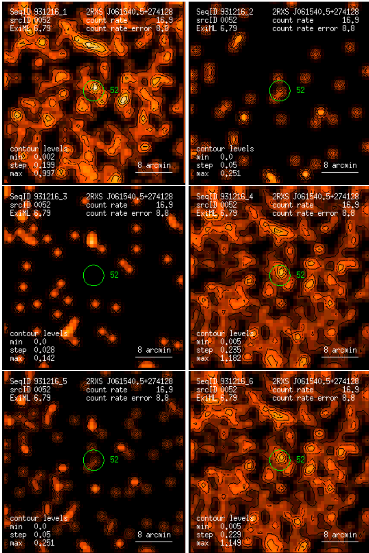
Figure 52: RASS 931216: detection 0052: band rate images, Gaussian filter: (1) PSPC channels 11 – 41, (2) 52 – 90, (3) 91 – 201, (4) 11 – 235, (5) 52 – 201, (6) 11 – 201. Broad band rates in counts/ks. Band rate contour levels in counts/ks/arcmin 2 .
