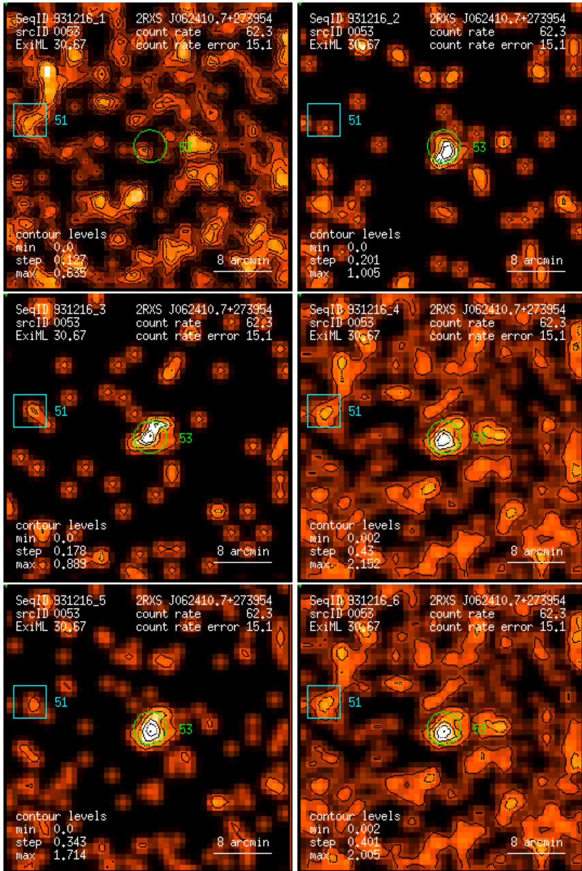
Figure 53: RASS 931216: detection 0053: band rate images, Gaussian filter: (1) PSPC channels 11 – 41, (2) 52 – 90, (3) 91 – 201, (4) 11 – 235, (5) 52 – 201, (6) 11 – 201. Broad band rates in counts/ks. Band rate contour levels in counts/ks/arcmin 2 .
