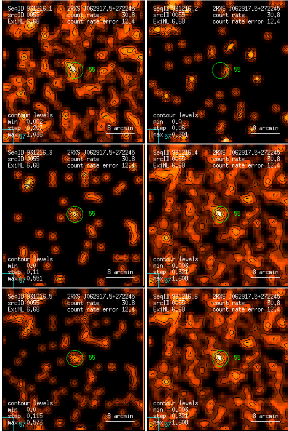
Figure 55: RASS 931216: detection 0055: band rate images, Gaussian filter: (1) PSPC channels 11 – 41, (2) 52 – 90, (3) 91 – 201, (4) 11 – 235, (5) 52 – 201, (6) 11 – 201. Broad band rates in counts/ks. Band rate contour levels in counts/ks/arcmin 2 .
