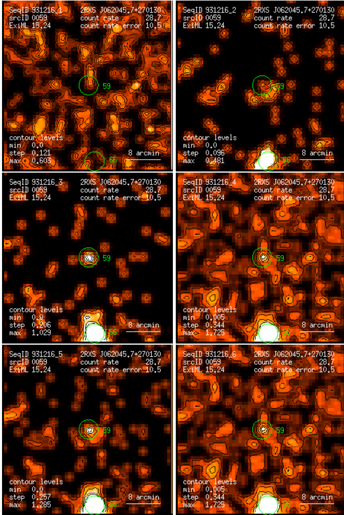
Figure 59: RASS 931216: detection 0059: band rate images, Gaussian filter: (1) PSPC channels 11 – 41, (2) 52 – 90, (3) 91 – 201, (4) 11 – 235, (5) 52 – 201, (6) 11 – 201. Broad band rates in counts/ks. Band rate contour levels in counts/ks/arcmin 2 .
