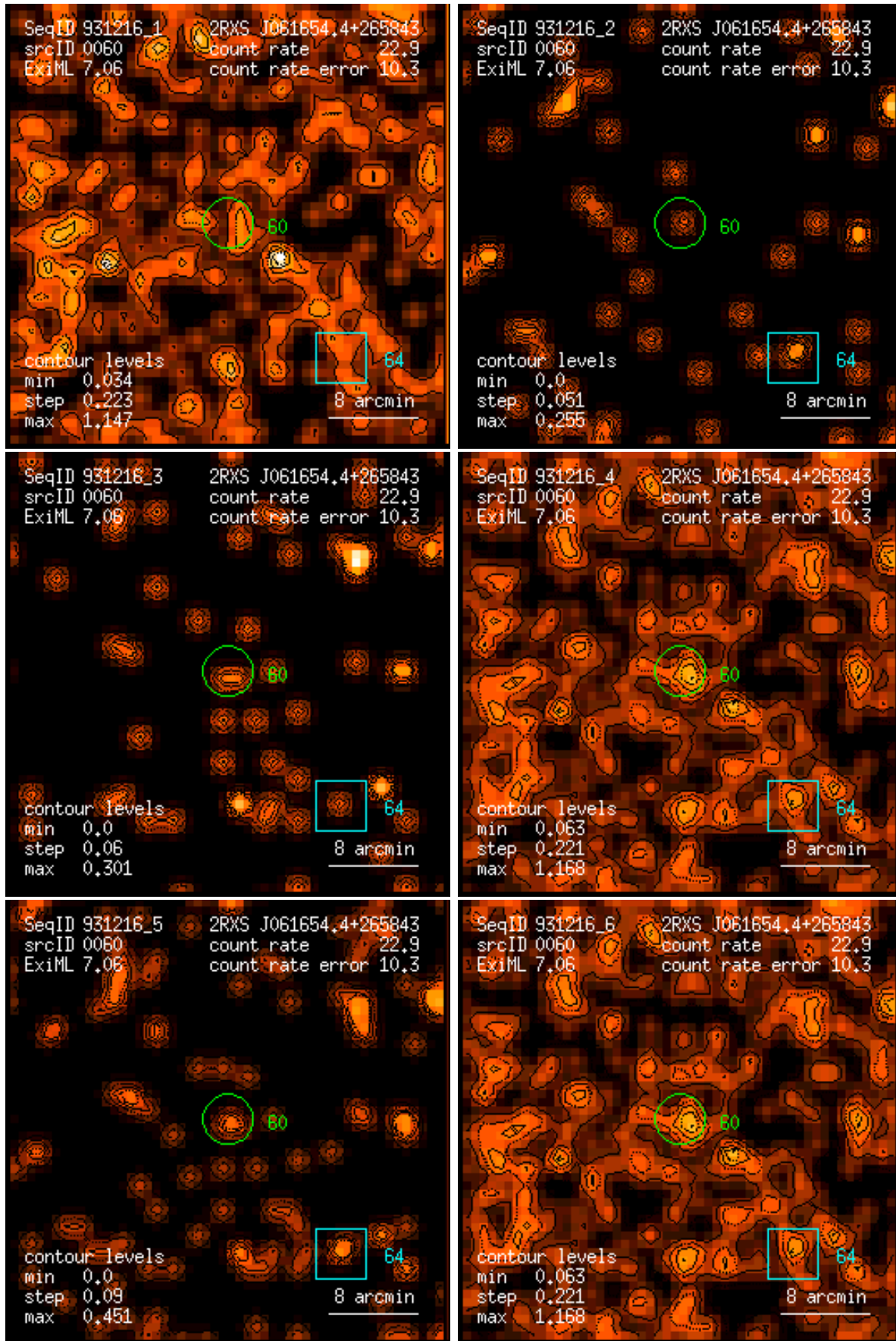
Figure 60: RASS 931216: detection 0060: band rate images, Gaussian filter: (1) PSPC channels 11 – 41, (2) 52 – 90, (3) 91 – 201, (4) 11 – 235, (5) 52 – 201, (6) 11 – 201. Broad band rates in counts/ks. Band rate contour levels in counts/ks/arcmin 2 .
