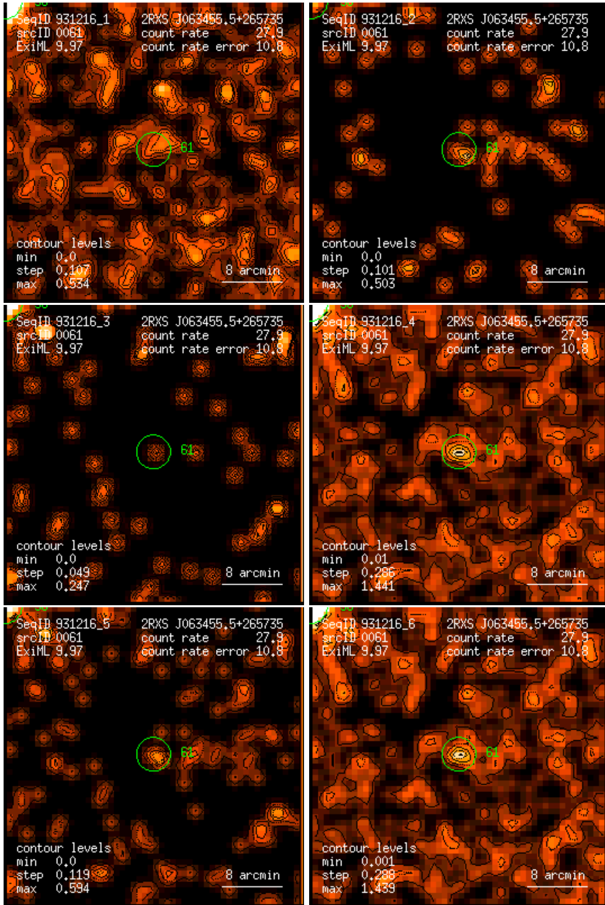
Figure 61: RASS 931216: detection 0061: band rate images, Gaussian filter: (1) PSPC channels 11 – 41, (2) 52 – 90, (3) 91 – 201, (4) 11 – 235, (5) 52 – 201, (6) 11 – 201. Broad band rates in counts/ks. Band rate contour levels in counts/ks/arcmin 2 .
