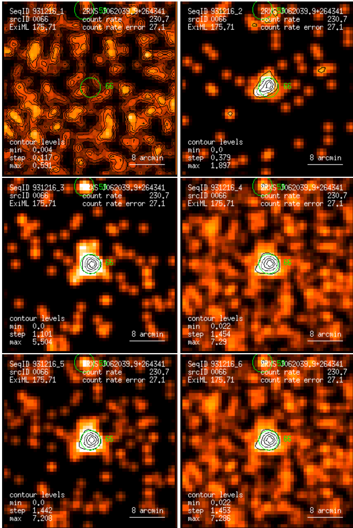
Figure 66: RASS 931216: detection 0066: band rate images, Gaussian filter: (1) PSPC channels 11 – 41, (2) 52 – 90, (3) 91 – 201, (4) 11 – 235, (5) 52 – 201, (6) 11 – 201. Broad band rates in counts/ks. Band rate contour levels in counts/ks/arcmin 2 .
