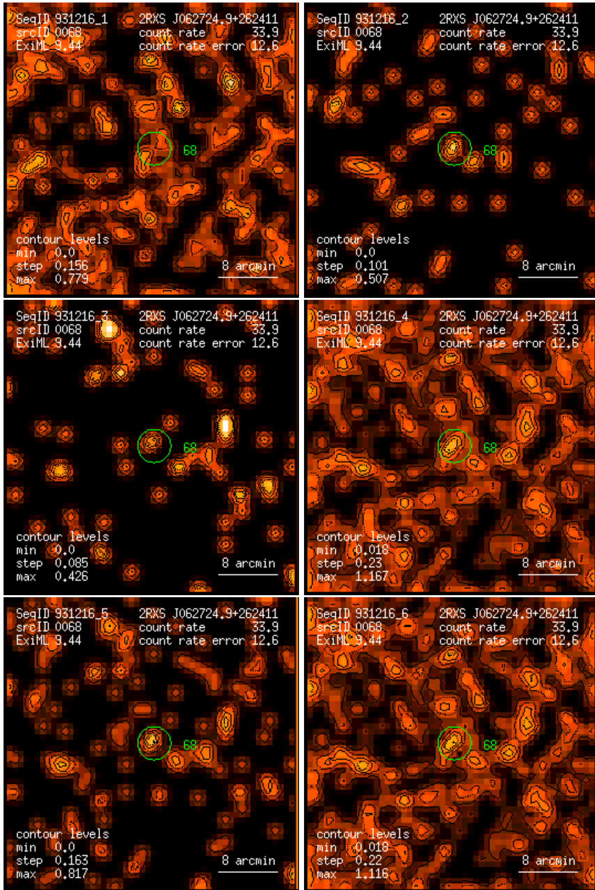
Figure 68: RASS 931216: detection 0068: band rate images, Gaussian filter: (1) PSPC channels 11 – 41, (2) 52 – 90, (3) 91 – 201, (4) 11 – 235, (5) 52 – 201, (6) 11 – 201. Broad band rates in counts/ks. Band rate contour levels in counts/ks/arcmin 2 .
