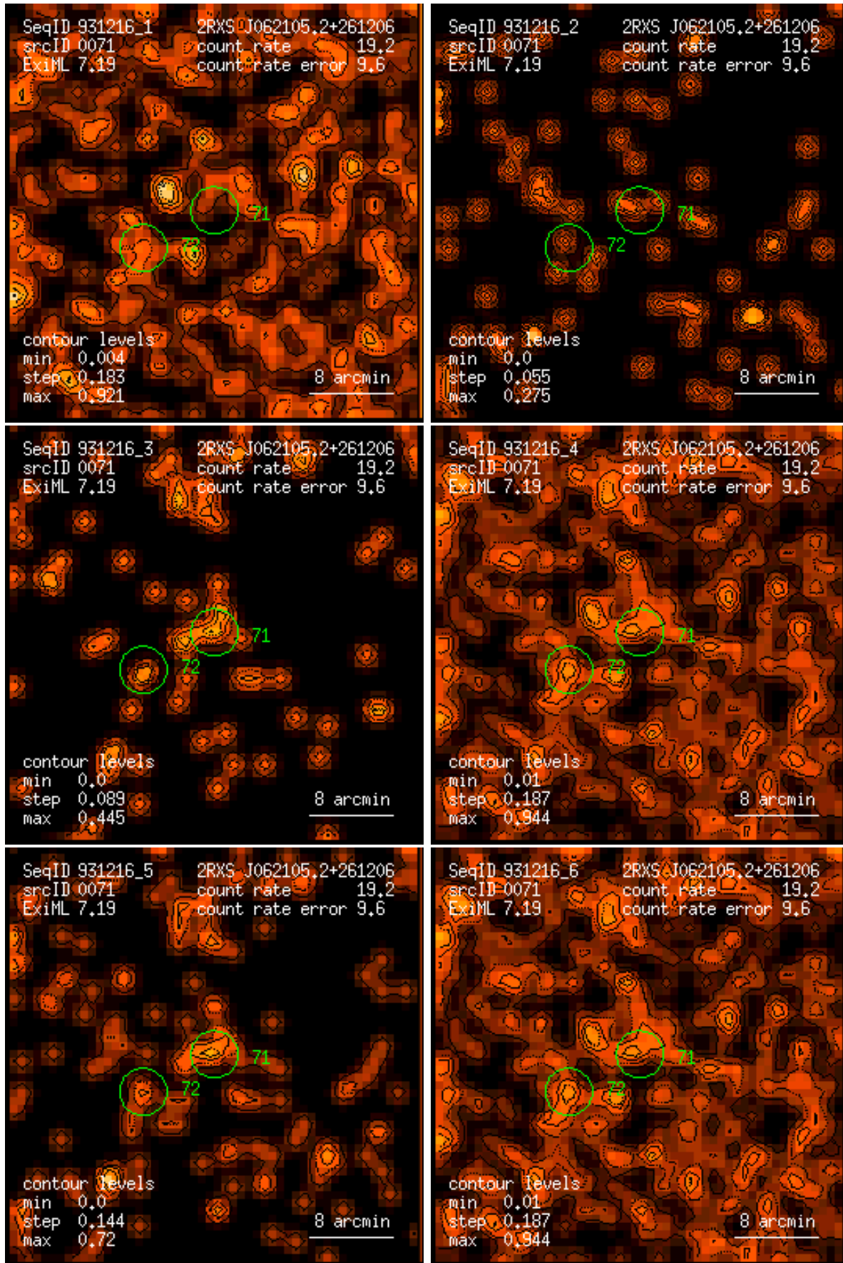
Figure 71: RASS 931216: detection 0071: band rate images, Gaussian filter: (1) PSPC channels 11 – 41, (2) 52 – 90, (3) 91 – 201, (4) 11 – 235, (5) 52 – 201, (6) 11 – 201. Broad band rates in counts/ks. Band rate contour levels in counts/ks/arcmin 2 .
