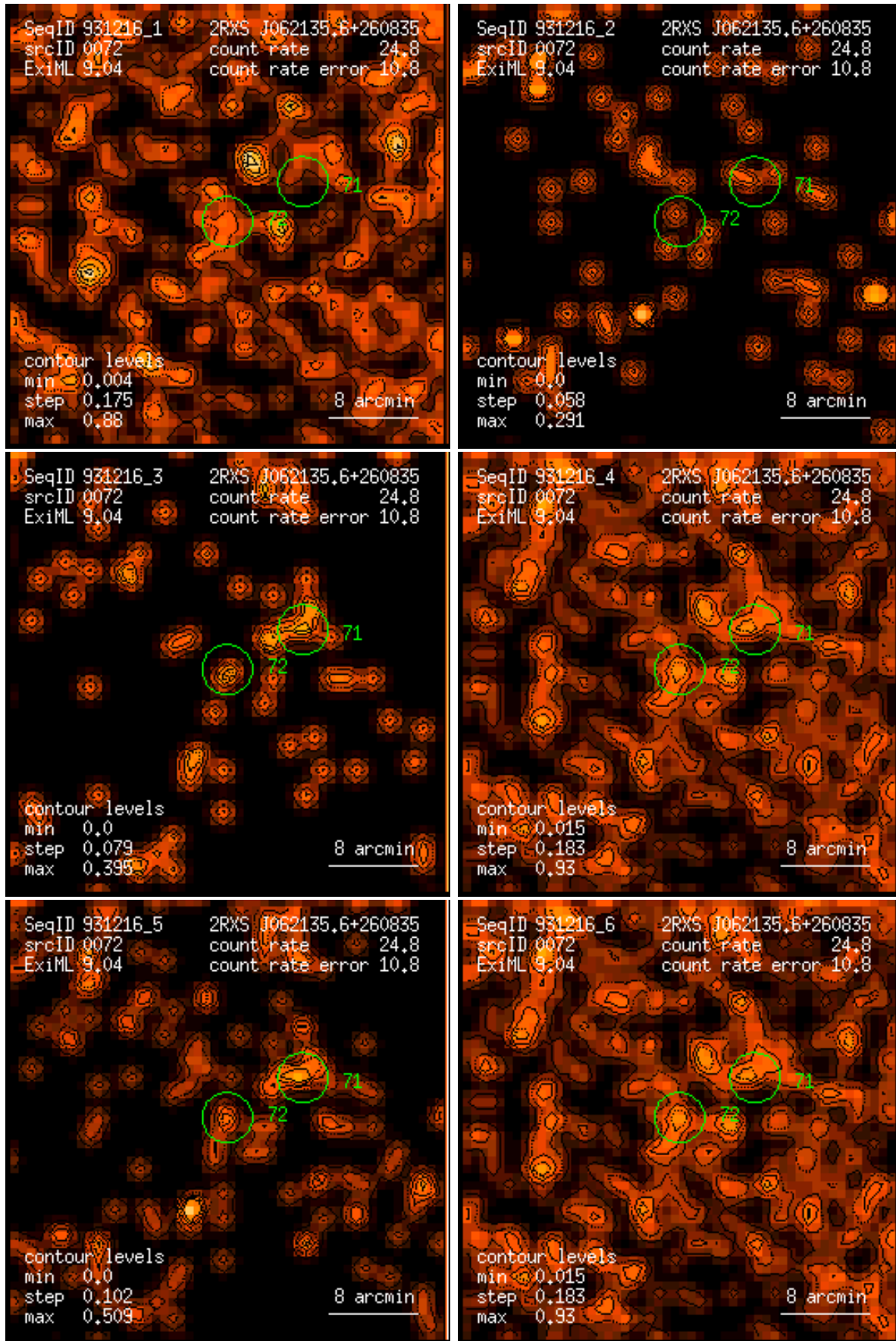
Figure 72: RASS 931216: detection 0072: band rate images, Gaussian filter: (1) PSPC channels 11 – 41, (2) 52 – 90, (3) 91 – 201, (4) 11 – 235, (5) 52 – 201, (6) 11 – 201. Broad band rates in counts/ks. Band rate contour levels in counts/ks/arcmin 2 .
