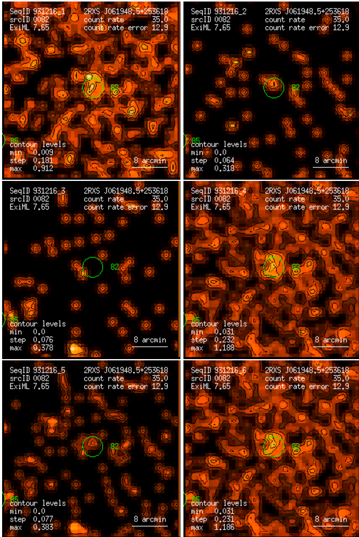
Figure 82: RASS 931216: detection 0082: band rate images, Gaussian filter: (1) PSPC channels 11 – 41, (2) 52 – 90, (3) 91 – 201, (4) 11 – 235, (5) 52 – 201, (6) 11 – 201. Broad band rates in counts/ks. Band rate contour levels in counts/ks/arcmin 2 .
