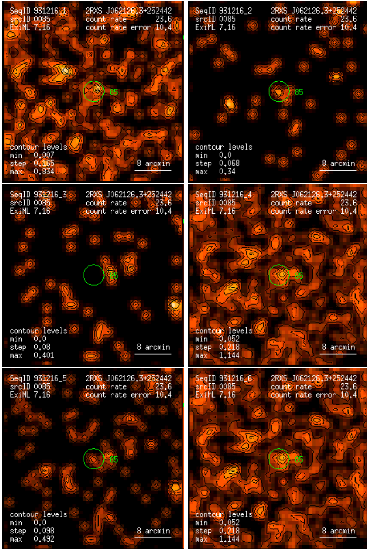
Figure 85: RASS 931216: detection 0085: band rate images, Gaussian filter: (1) PSPC channels 11 – 41, (2) 52 – 90, (3) 91 – 201, (4) 11 – 235, (5) 52 – 201, (6) 11 – 201. Broad band rates in counts/ks. Band rate contour levels in counts/ks/arcmin 2 .
