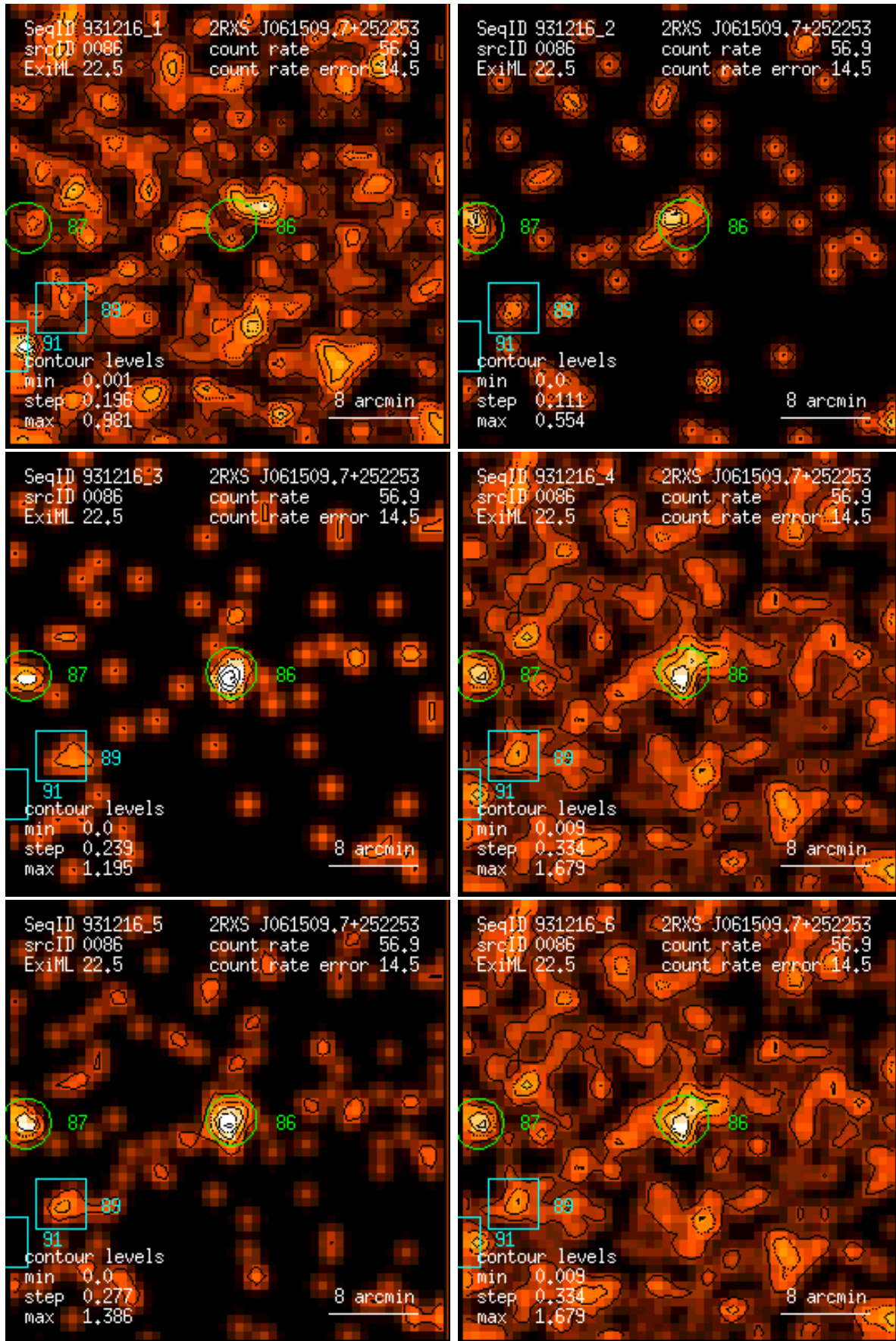
Figure 86: RASS 931216: detection 0086: band rate images, Gaussian filter: (1) PSPC channels 11 – 41, (2) 52 – 90, (3) 91 – 201, (4) 11 – 235, (5) 52 – 201, (6) 11 – 201. Broad band rates in counts/ks. Band rate contour levels in counts/ks/arcmin 2 .
