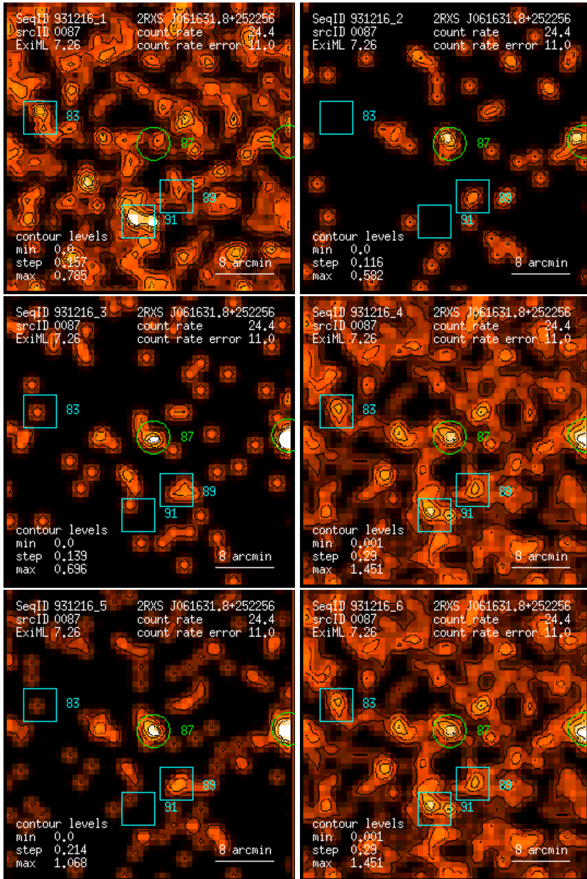
Figure 87: RASS 931216: detection 0087: band rate images, Gaussian filter: (1) PSPC channels 11 – 41, (2) 52 – 90, (3) 91 – 201, (4) 11 – 235, (5) 52 – 201, (6) 11 – 201. Broad band rates in counts/ks. Band rate contour levels in counts/ks/arcmin 2 .
