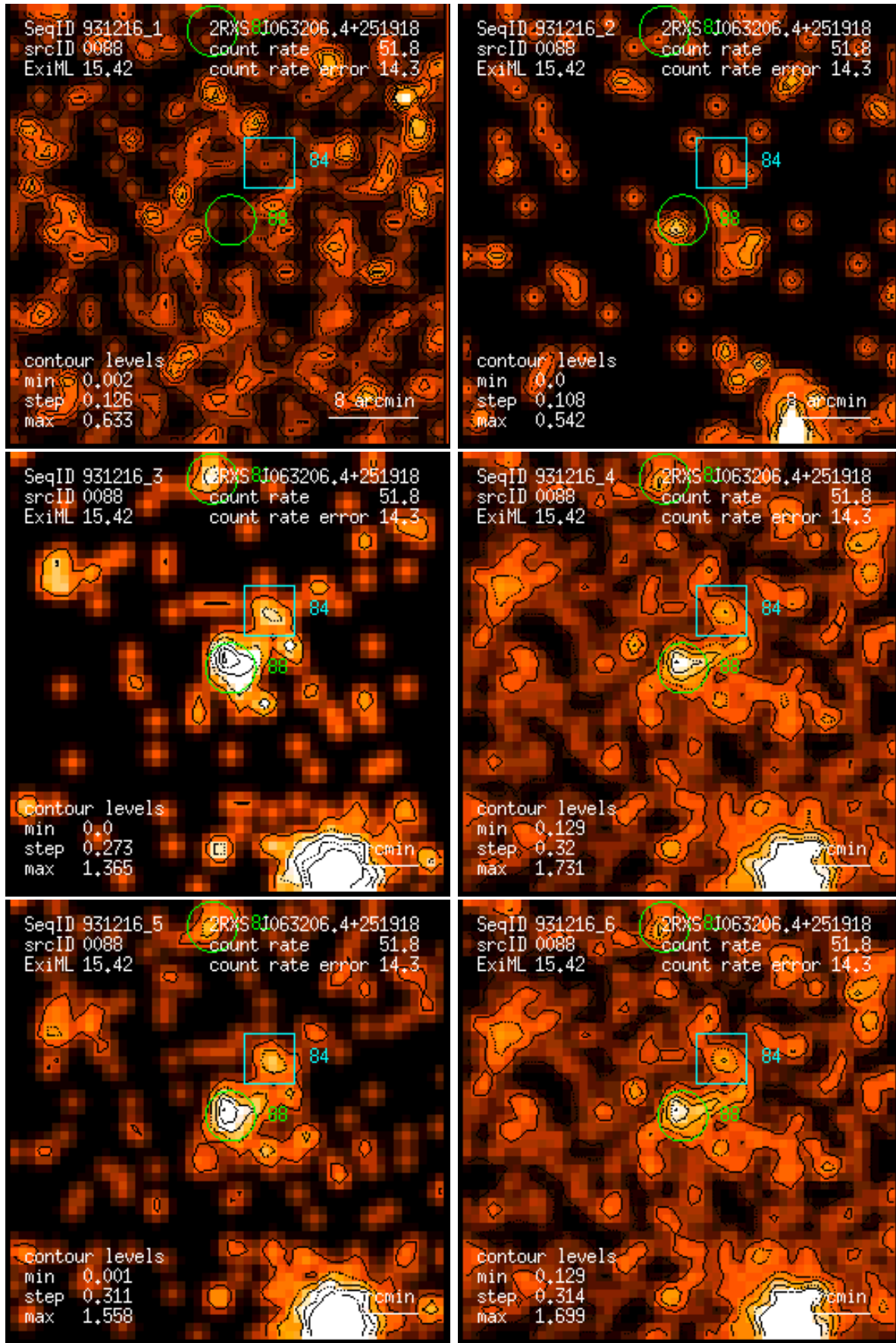
Figure 88: RASS 931216: detection 0088: band rate images, Gaussian filter: (1) PSPC channels 11 – 41, (2) 52 – 90, (3) 91 – 201, (4) 11 – 235, (5) 52 – 201, (6) 11 – 201. Broad band rates in counts/ks. Band rate contour levels in counts/ks/arcmin 2 .
