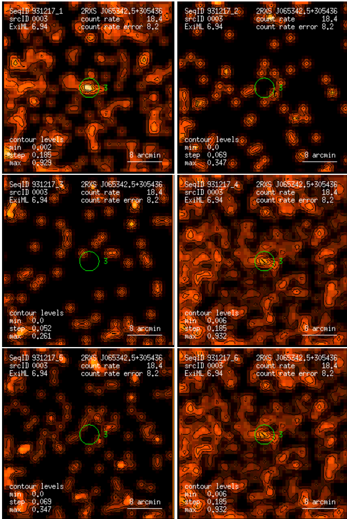
Figure 3: RASS 931217: detection 0003: band rate images, Gaussian filter: (1) PSPC channels 11 – 41, (2) 52 – 90, (3) 91 – 201, (4) 11 – 235, (5) 52 – 201, (6) 11 – 201. Broad band rates in counts/ks. Band rate contour levels in counts/ks/arcmin 2 .
