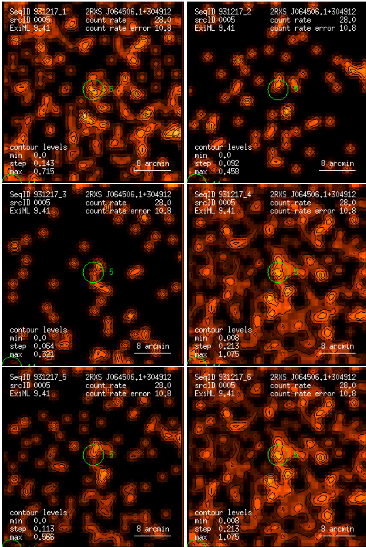
Figure 5: RASS 931217: detection 0005: band rate images, Gaussian filter: (1) PSPC channels 11 – 41, (2) 52 – 90, (3) 91 – 201, (4) 11 – 235, (5) 52 – 201, (6) 11 – 201. Broad band rates in counts/ks. Band rate contour levels in counts/ks/arcmin 2 .
