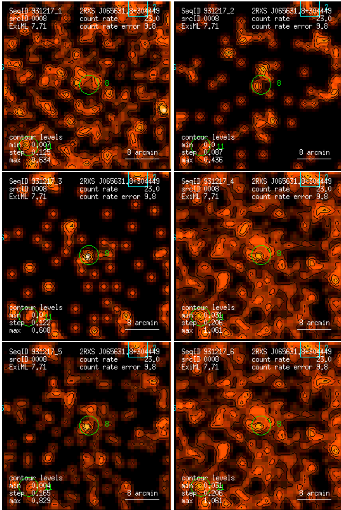
Figure 8: RASS 931217: detection 0008: band rate images, Gaussian filter: (1) PSPC channels 11 – 41, (2) 52 – 90, (3) 91 – 201, (4) 11 – 235, (5) 52 – 201, (6) 11 – 201. Broad band rates in counts/ks. Band rate contour levels in counts/ks/arcmin 2 .
