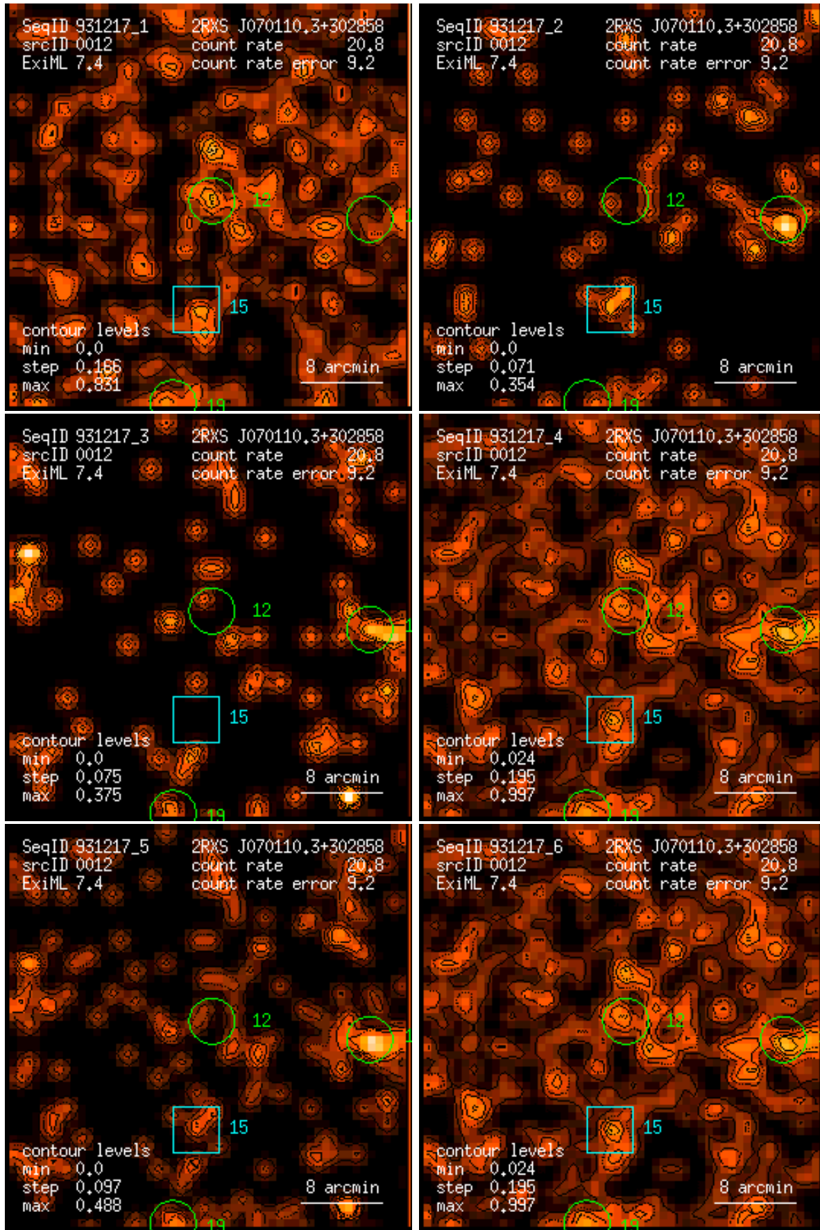
Figure 12: RASS 931217: detection 0012: band rate images, Gaussian filter: (1) PSPC channels 11 – 41, (2) 52 – 90, (3) 91 – 201, (4) 11 – 235, (5) 52 – 201, (6) 11 – 201. Broad band rates in counts/ks. Band rate contour levels in counts/ks/arcmin 2 .
